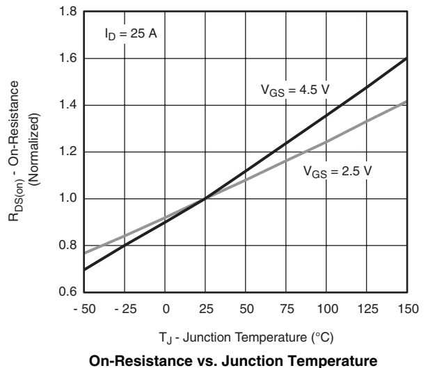
I_D = 25 \text{ A} V_{GS} = 4.5 \text{ V} V_{GS} = 2.5 \text{ V} On-Resistance vs. Junction Temperature
