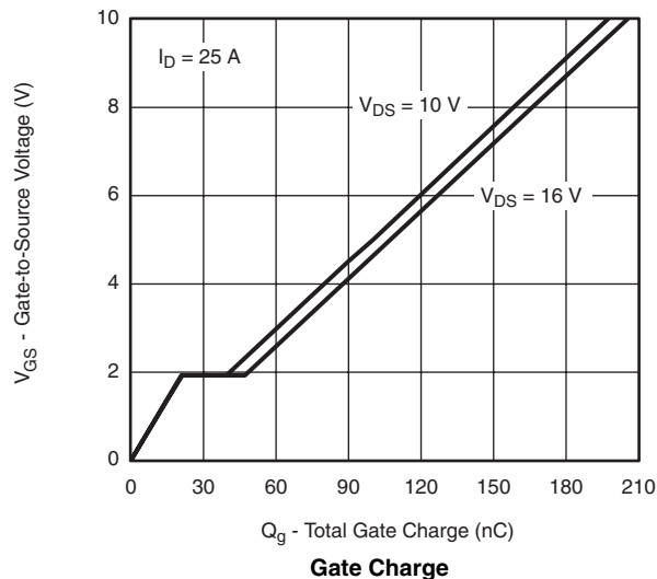
I_D = 25 \text{ A} V_{DS} = 10 \text{ V} V_{DS} = 16 \text{ V} Gate Charge
