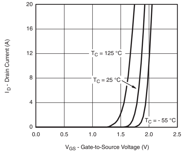
T_C = 125^\circ\text{C} T_C = 25^\circ\text{C} T_C = -55^\circ\text{C} Transfer Characteristics
