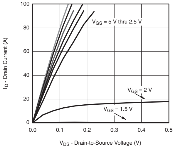
V_{GS} = 5 \text{ V thru } 2.5 \text{ V} Output Characteristics
