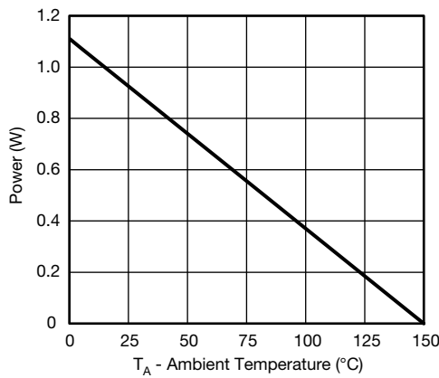
Power, Junction-to-Ambient
