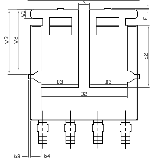
BACKSIDE VIEW(DUAL)
